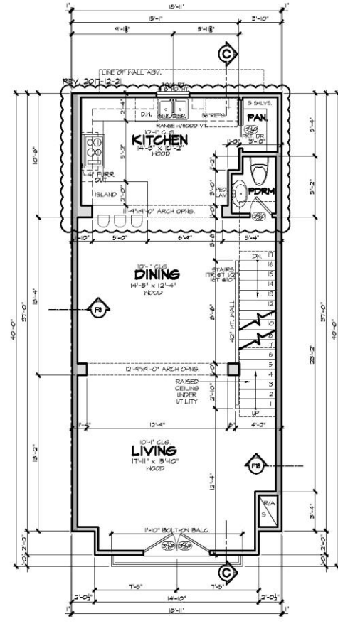
SECOND FLOOR PLAN SCALE: 1/4" = 1'-0" 10'-0" CEILINGS UND. PRIMARY FLOOR COVERINGS: HOOD UND. SUGGESTED FLOOR SYSTEM: 18" TRUSSES
