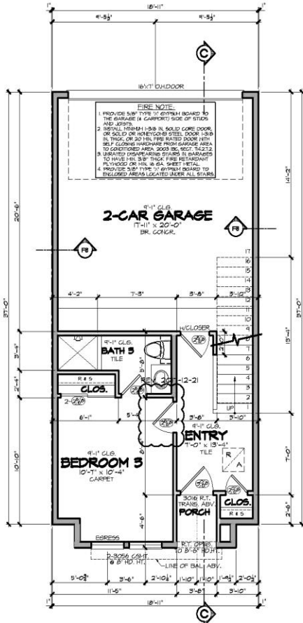
FIRST FLOOR PLAN SCALE: 1/4" = 1'-0" 8'-0" CEILINGS UND. PRIMARY FLOOR COVERINGS: CARPET UND.
