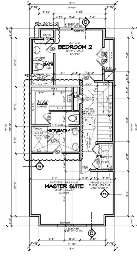
THIRD FLOOR PLAN SCALE: 1/4" = 1'-0" 8'-0" CEILINGS UND. PRIMARY FLOOR COVERINGS: CARPET UND. SUGGESTED FLOOR SYSTEM: 18" TRUSSES PROVIDE METAL PAN W/2" DRAIN TO OUTSIDE IN UTILITY AREA
