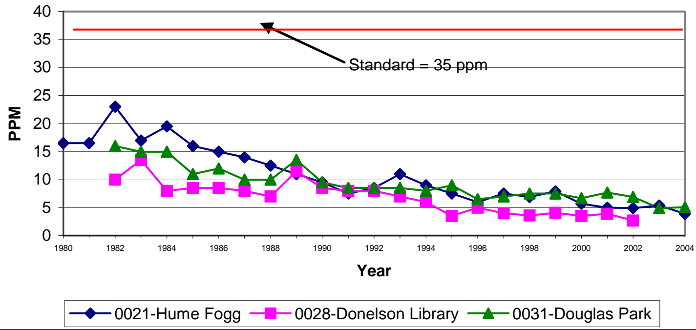
ANNUAL COMPARISON CARBON MONOXIDE CONCENTRATIONS (PPM) Highest 1-Hour Concentrations Figure 13
