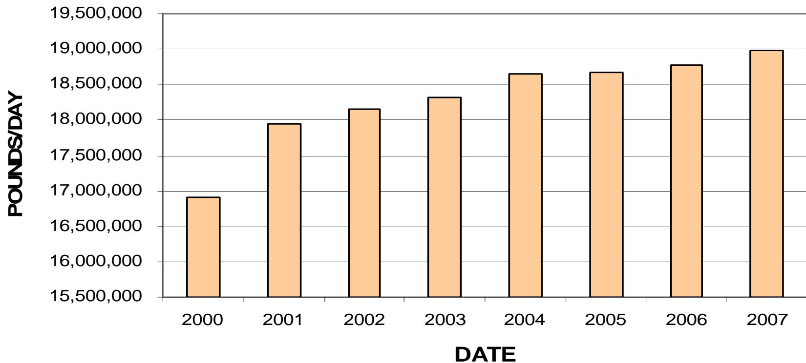
2007 ESTIMATED DAILY CO2 EMISSIONS FROM LDGV IN DAVIDSON COUNTY (~19 # CO2/GALLON BURNED)
