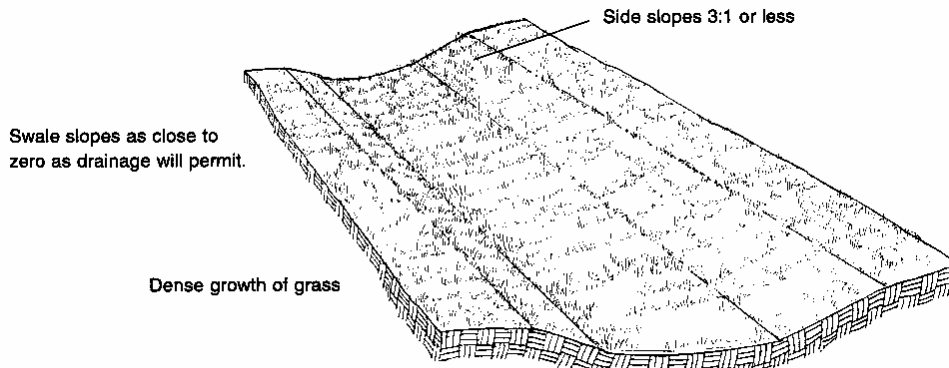
Figure 8.1 Typical Grass Channel
