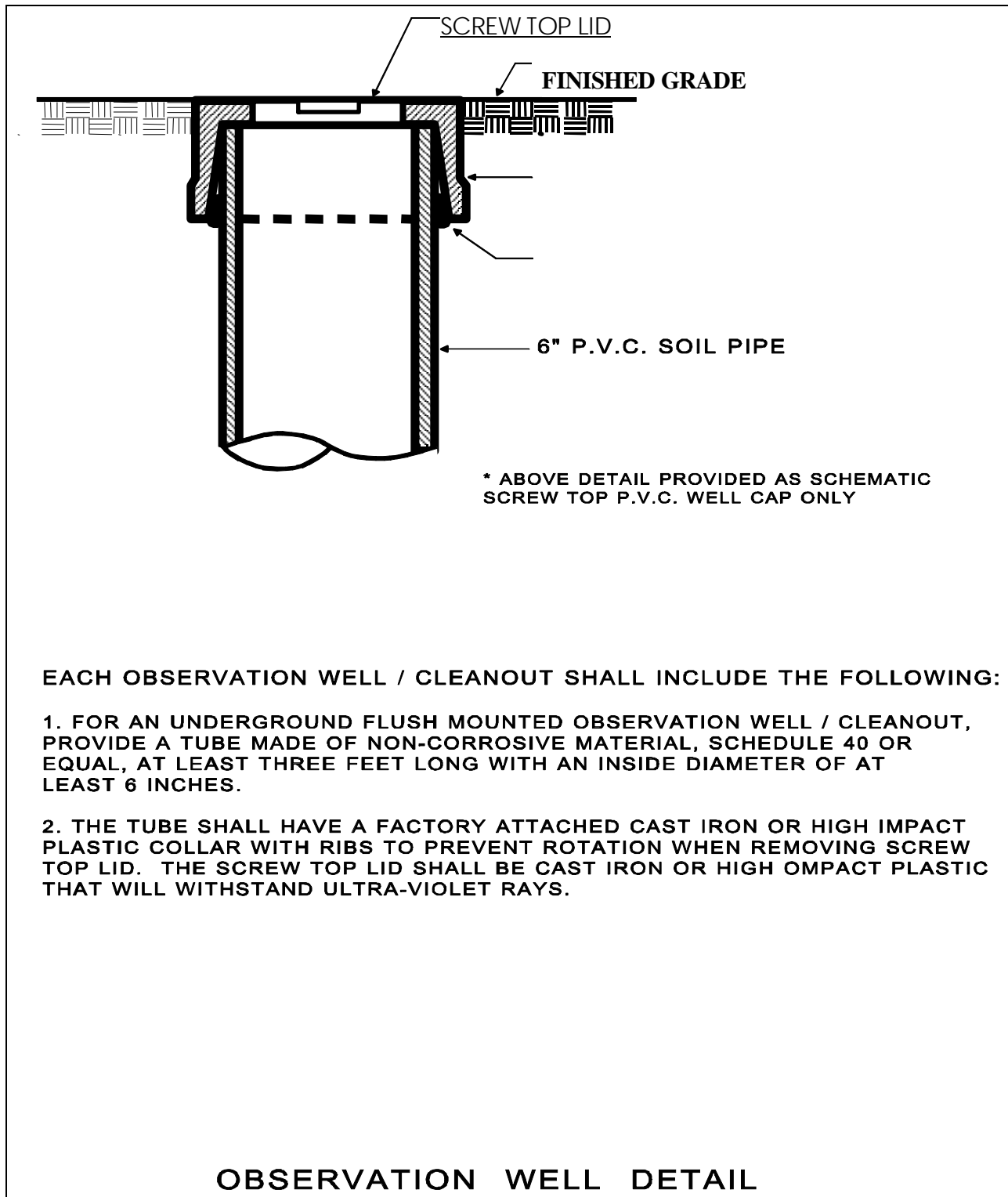
Figure 14.3 Observation Well Detail
