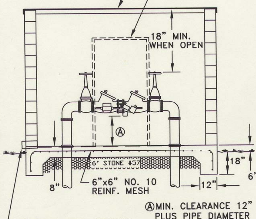
SIDE SECTION
