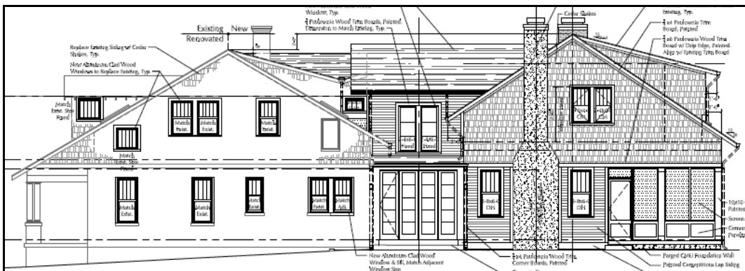
Figure 4: North elevation. Note the differing eave heights.
