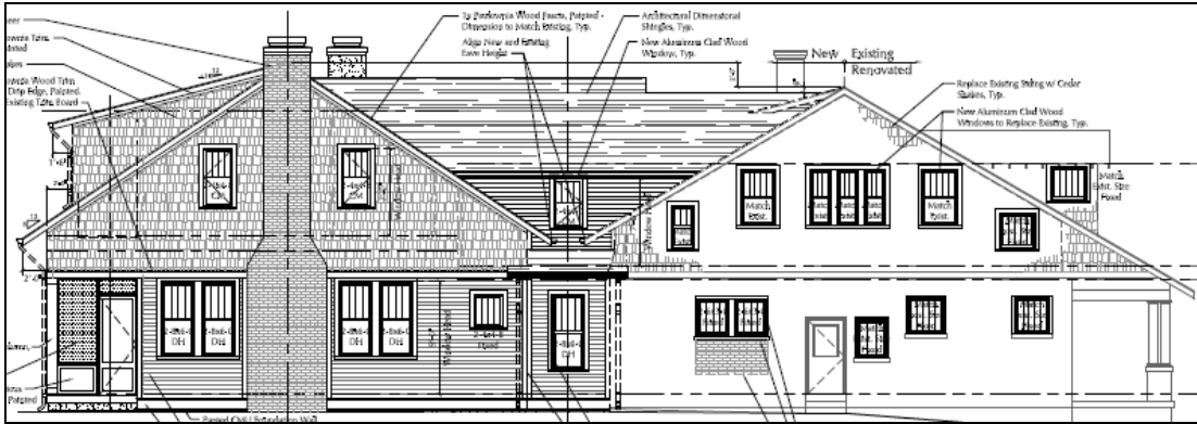
Figure 3: Ashwood Avenue elevation
