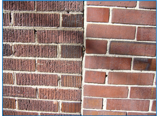
Preserve and maintain historic masonry.
