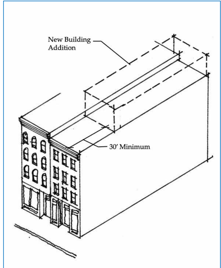
Required setbacks for a one-story rooftop addition.
