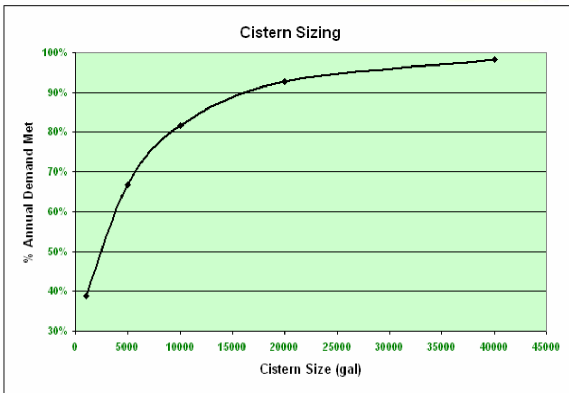
Figure 3.14--Cistern Sizing Example.
