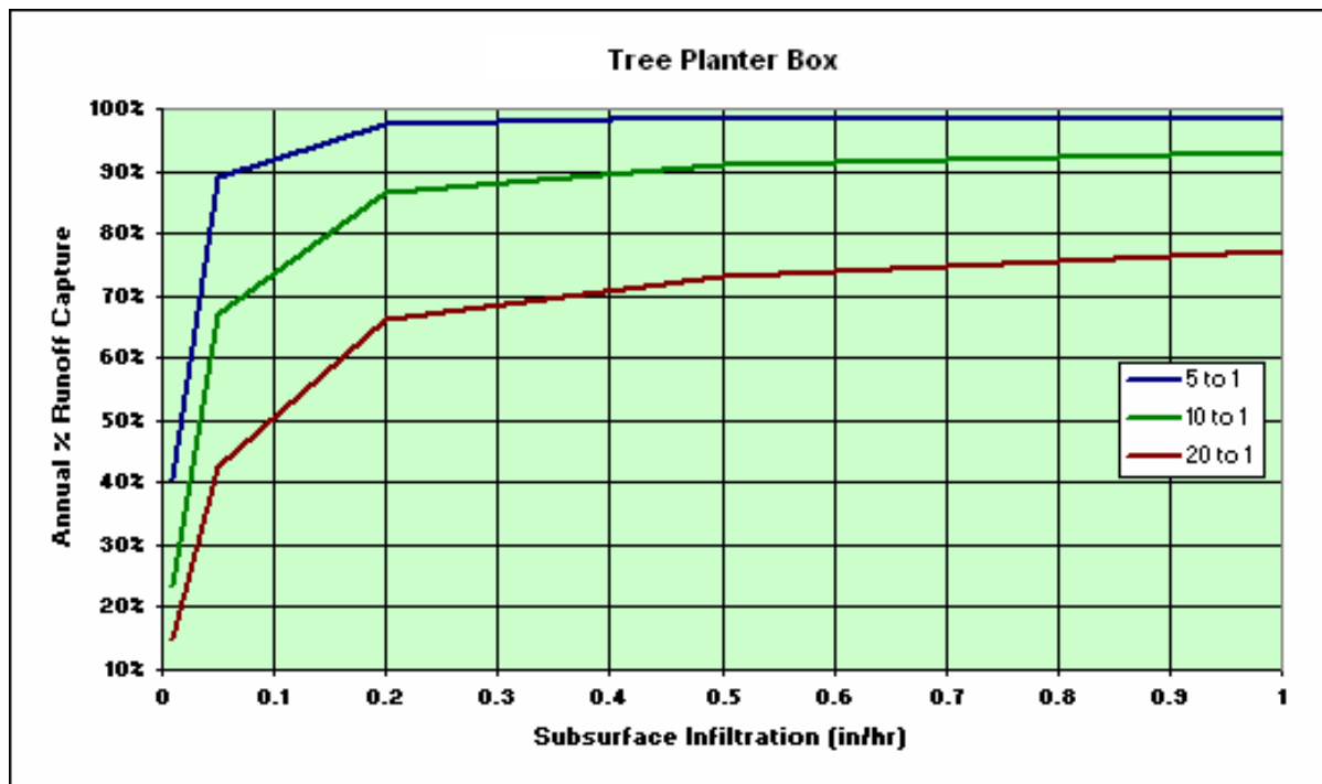
Figure 3.42--Tree Planter Box Modeling Results.
