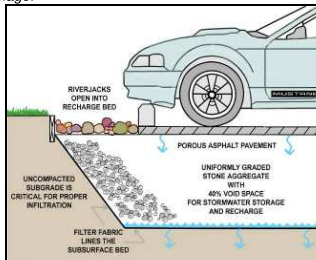
Permeable Pavement Cross-section Source: Cahill Associates
