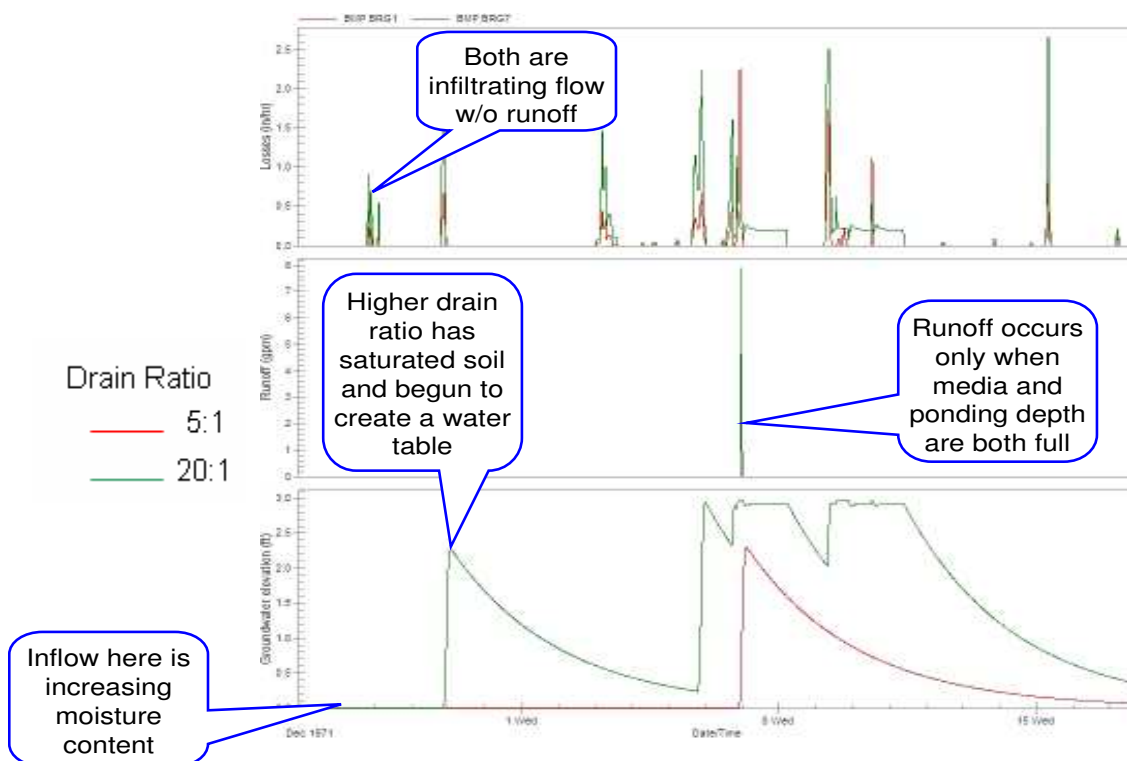
Figure 3.31--Results for 3' Deep Bioretention Cells with Underlying Percolation of 0.2"/hr.
