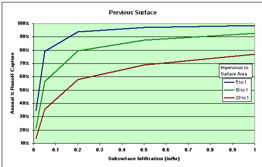
Figure 3.39--Pervious Surface Modeling Results, Media = 2.5' Gravel.
