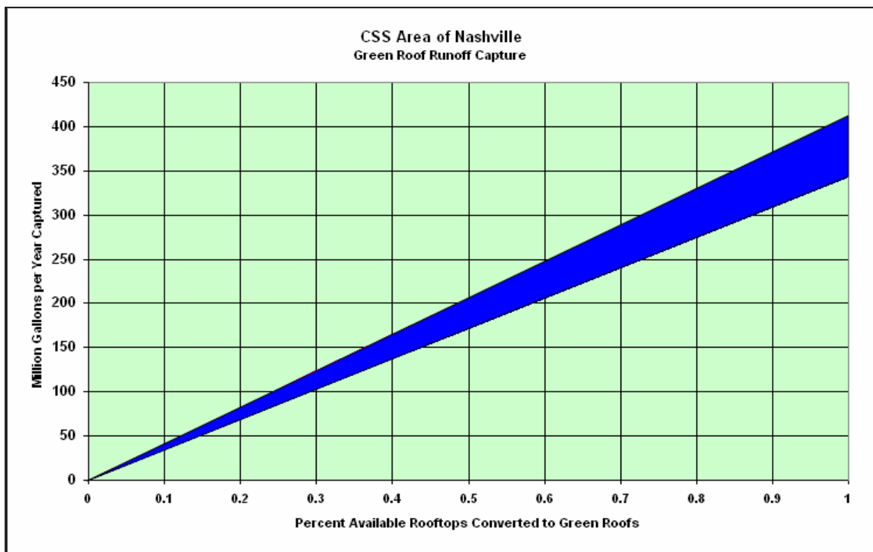
Figure 3.19—Potential Runoff Capture by Flat Roof Conversion to Green Roofs.
