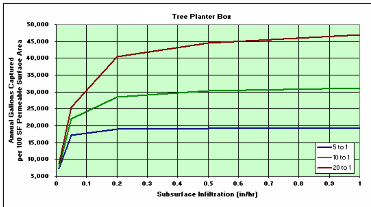
Figure 3.43--Annual Gallons Removed for 6' by 6' Planter Boxes.
