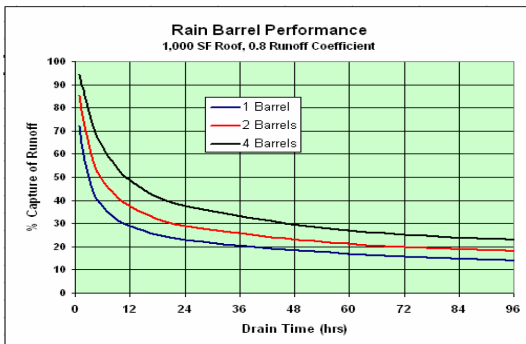
Figure 3.12—Runoff Capture of Various Rain Barrel Configurations.
