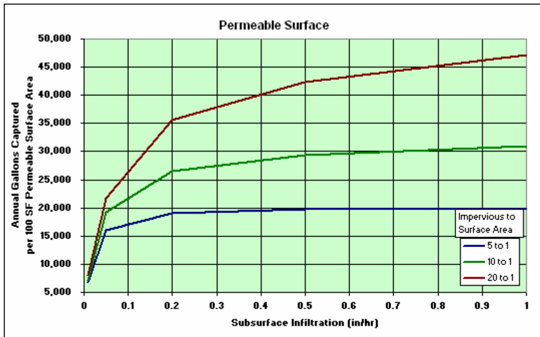
Figure 3.40--Annual Gallons Removed for Pervious Surfaces.
