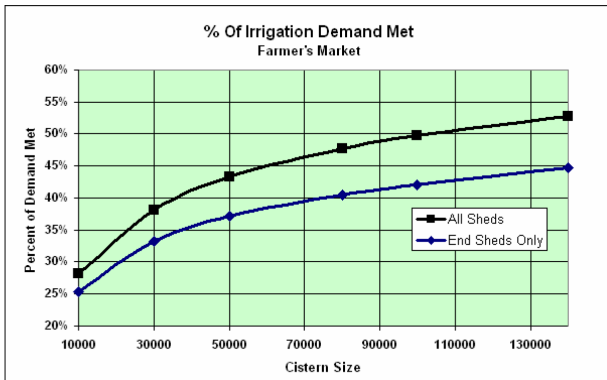
Figure 3.15—Cistern sizing for Farmer's Market.
