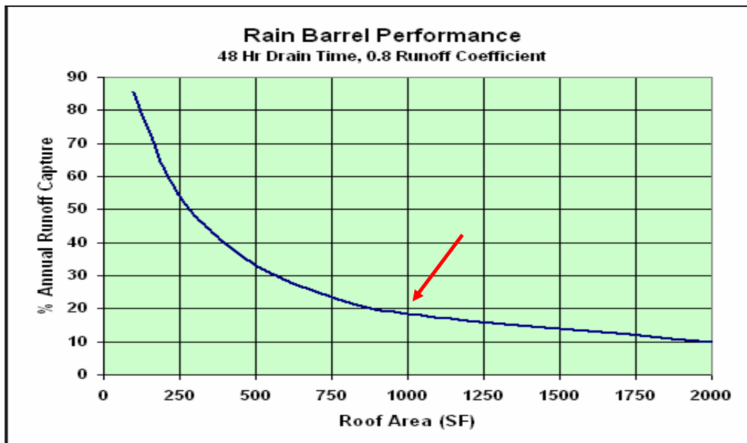
Figure 3.13--Rain Barrel Capture Efficiency Based on Roof Area.
