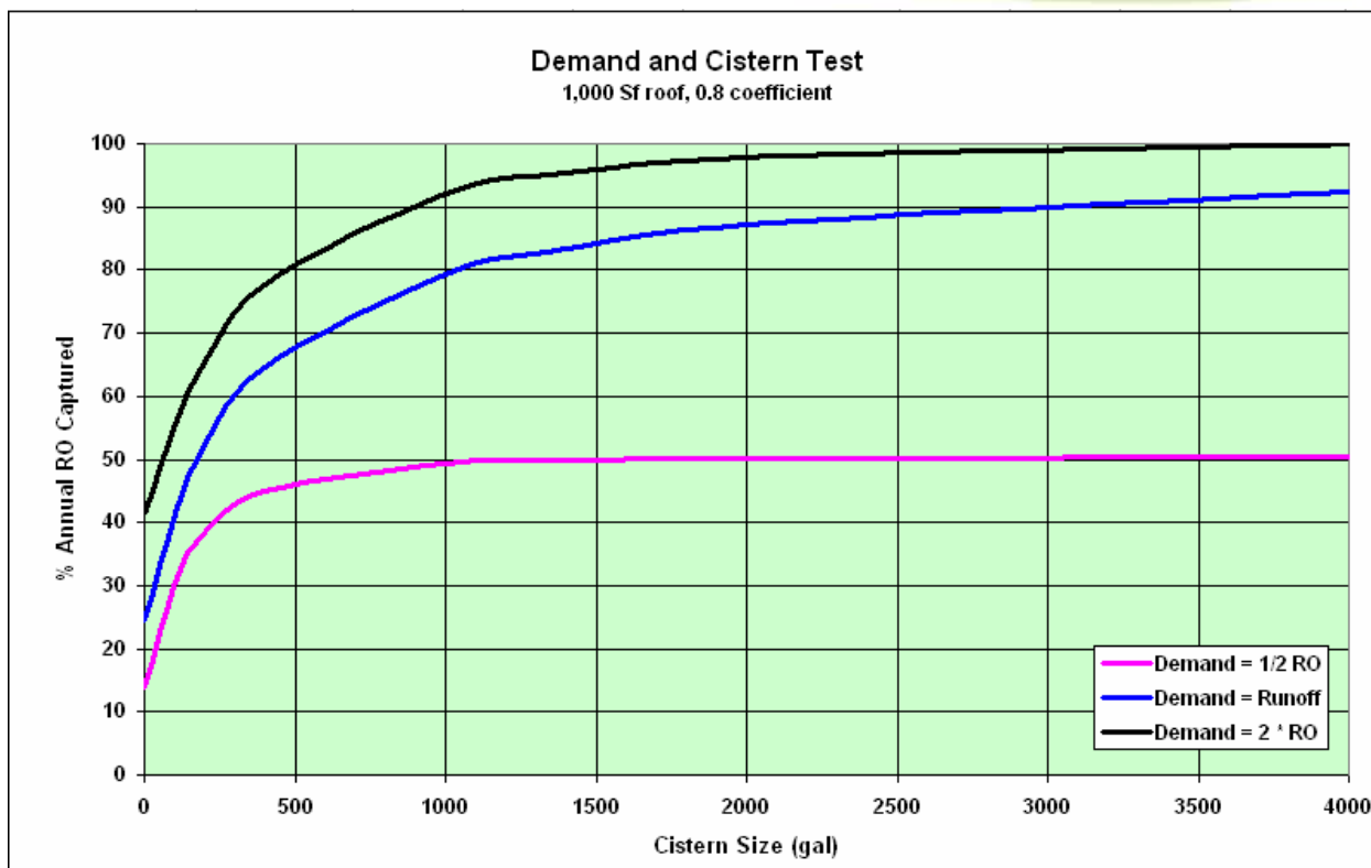
Figure 3.9—Cistern Test for Three Demand Conditions.
