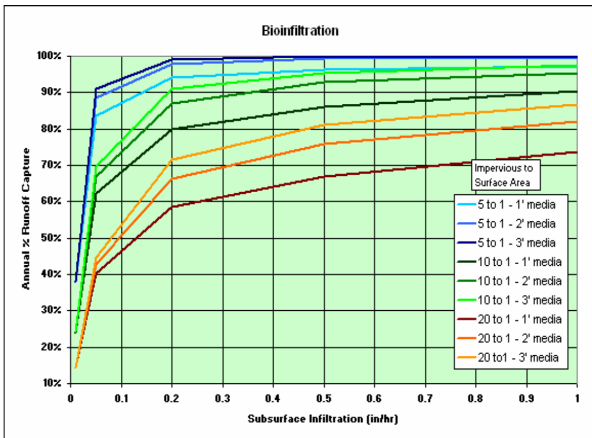
Figure 3.34--Bioinfiltration Modeling Results.
