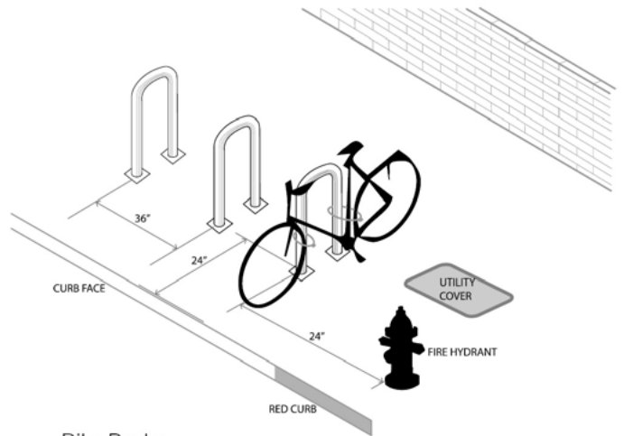
Bike Racks
