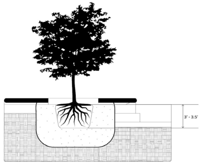
Soil Depth
